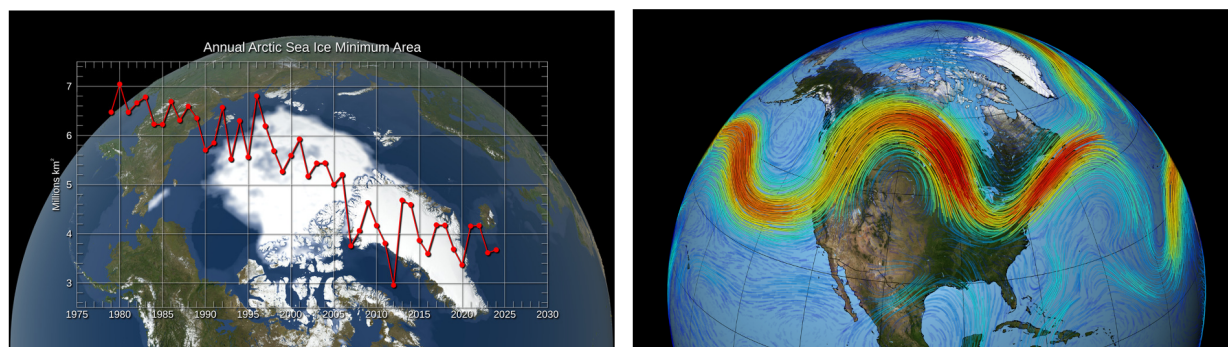
Figure 4: Left: Arctic minimum sea ice extent from 1979-2024, showing a declining trend in ice cover over the last 4.5 decades resulting in a significantly greater exposure of ocean water to the atmosphere. Right: Atmospheric circulation patterns showing the linkage between the high-latitude regions and the United States. Images courtesy of NASA (Right and left images are ( https://svs.gsfc.nasa.gov/5395/ and ( https://svs.gsfc.nasa.gov/3864 respectively).
