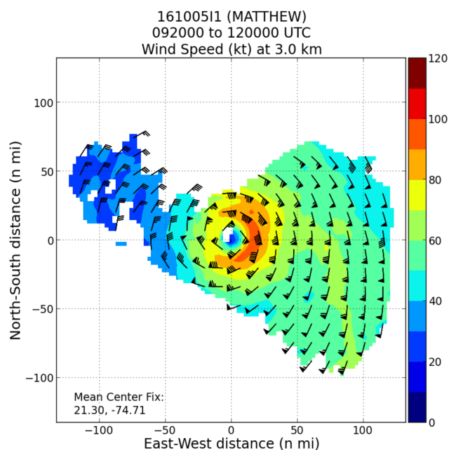
Figure 3: Left: Aircraft tail doppler-derived winds during Hurricane Matthew in 2016 (AOML, 2016); Right: Natural color image acquired by the Moderate Resolution Imaging Spectroradiometer (MODIS) on NASA's Terra satellite (NASA Goddard, 2016). While the MODIS image clearly shows the extent of the hurricane, the bands and the cloud cover, the doppler image shows the strength and windspeed and provides precipitation. Together they provide a comprehensive depiction of the hurricane structure, extent, precipitation, winds and trajectory.
